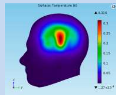
The local temperature distribution in brain region of human head model at 900MHz.
